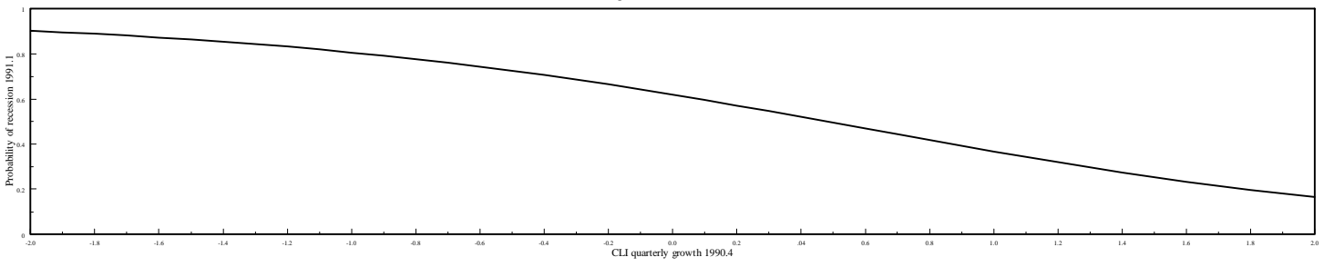
Graph 2. KERNEL simulation
