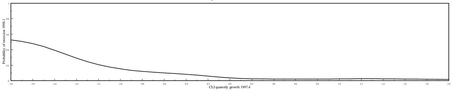
Graph 3. RTCOMB simulation
