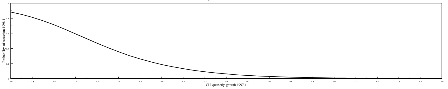
Graph 2. KERNEL simulation
