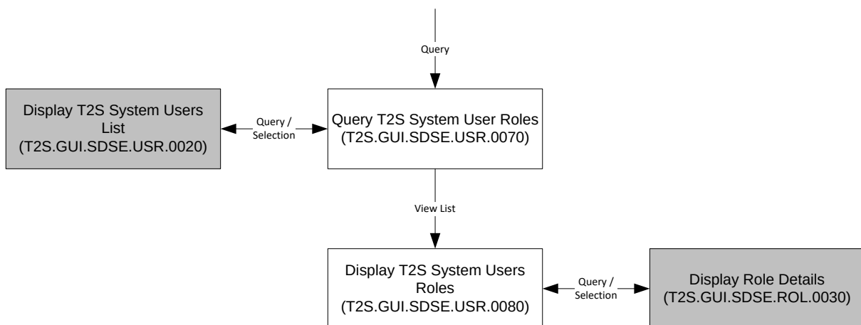
Figure 4-52 T2S System User Roles Query user interface framework
